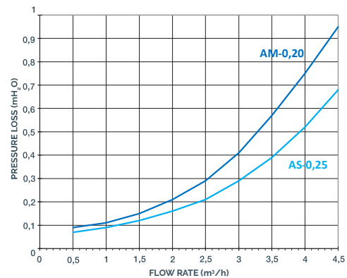
NOZZLE AM - AS
